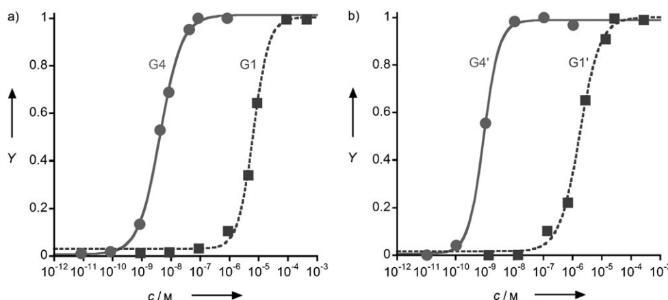
Figure 3. Hill plot of a) copolymers G1, G4 and b) homopolymers G1', G4' in EYPC:CF vesicles with fits to the Hill equation.
