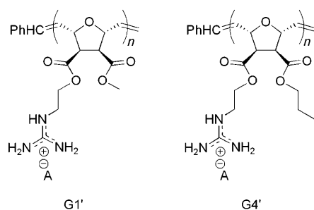
Scheme 2. Guanidino homopolymers G1' and G4'.
