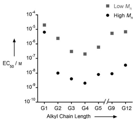
Figure 1. Effective concentrations ( EC_{50} ) of low-molecular-weight and high-molecular-weight copolymers G1–G12 as a function of alkyl side-chain length.
