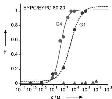
Figure 2. Hill plot for copolymers G1 and G4 in EYPC/EYPG⊃CF vesicles with fits to the Hill equation (circles). G1 EC_{50} = 0.4 \mu\text{M} , G4 EC_{50} = 0.04 \mu\text{M} . G1 and G4 remained inactive against EYPC/EYPG⊃calcein vesicles (triangles).
